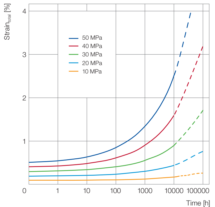
Fig. 20: Creep curves according to ISO 899 for Ultrason® E 2010 G6 at 180 °C
