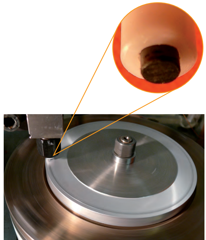
Fig. 23: Wear behavior Tribological system: pin-on-disk apparatus, surface pressure p = 1 \text{ MPa} , base material aluminum with 6.7 \text{ µm} roughness (dry)
