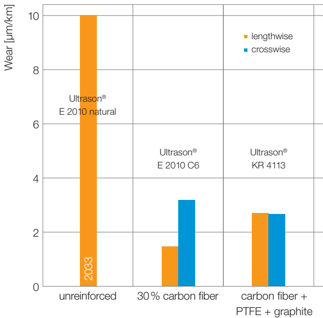
Fig. 23: Wear behavior Tribological system: pin-on-disk apparatus, surface pressure p = 1 \text{ MPa} , base material aluminum with 6.7 \text{ µm} roughness (dry)
