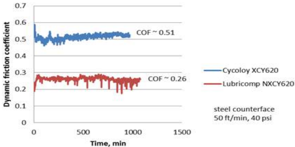
COF with and without silicone
