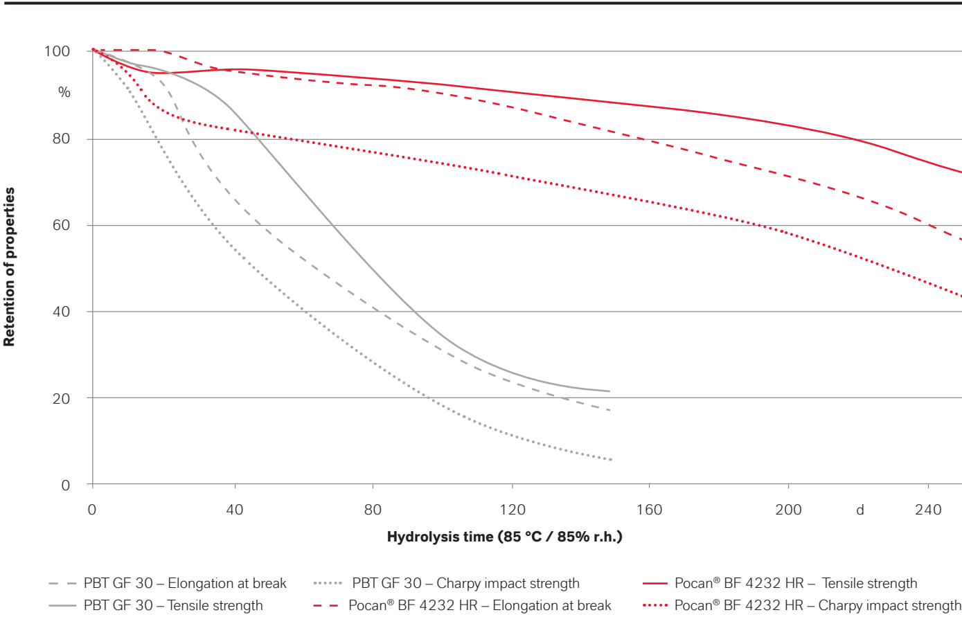
Fig. 5: Reduction of impact strength, tensile strength and elongation at break after storage at 85 °C and 85% rel. humidity: even after 200 days, the mechanical properties of Pocan® BF 4232 HR are still at a very high level compared to a standard PBT with a glass fiber content of 30%
