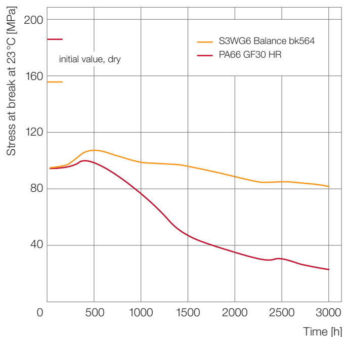
Abb. 24: Hydrolysis resistance of Ultramid® S Balance compared with PA66, in Glycantin/water (1:1) at 130°C
