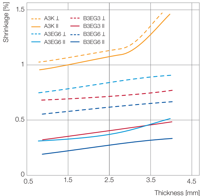
Fig. 37: Impeded shrinkage of different Ultramid® grades as a function of wall thickness (sheet measuring 110 x 110 mm made using a film gate; P_N=500 bar; ⊥ means perpendicular and II means parallel to the melt flow direction)
