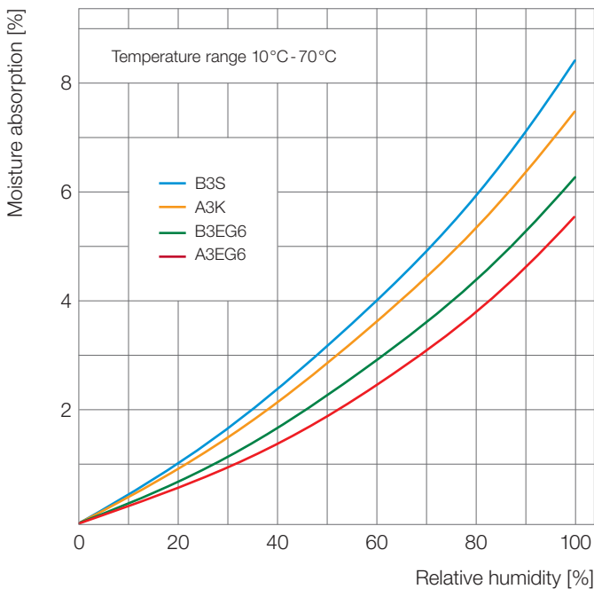
Fig. 16: Equilibrium moisture content of Ultramid® as a function of relative humidity in the temperature range 10°C-70°C (scatter: \pm 0.2 to 0.4% absolute)
